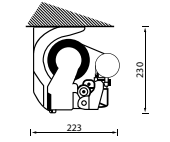
Ceiling/Top fix with Global 2020 bracket
