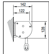
Wall Installation
