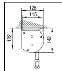
Ceiling Installation
